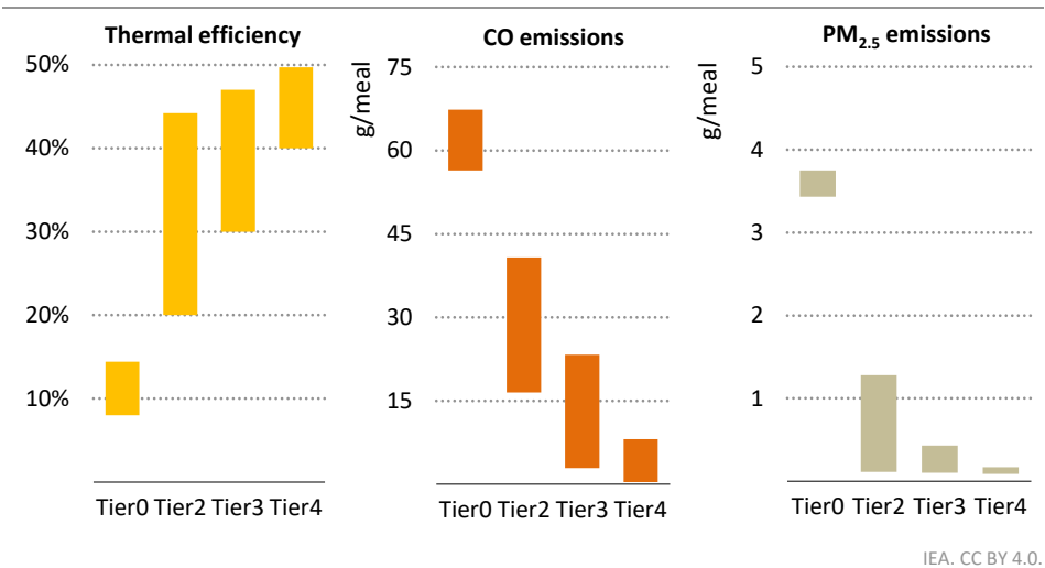
Figure 2.15 ▶ Range of thermal efficiencies and harmful emissions from different biomass stoves by Tier.
