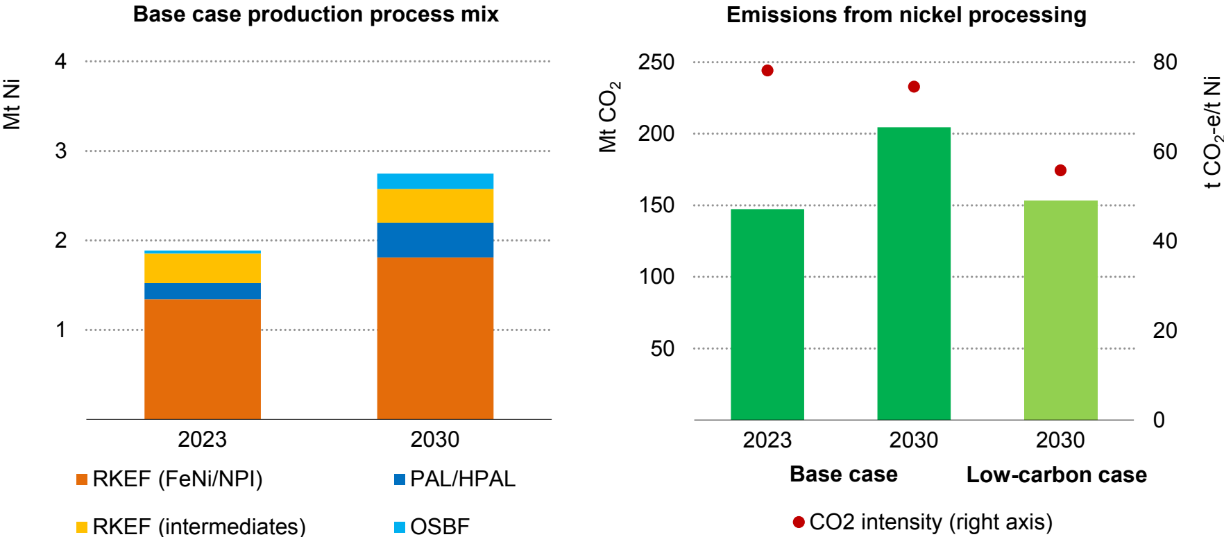
Indonesia nickel processing volumes and associated emissions
