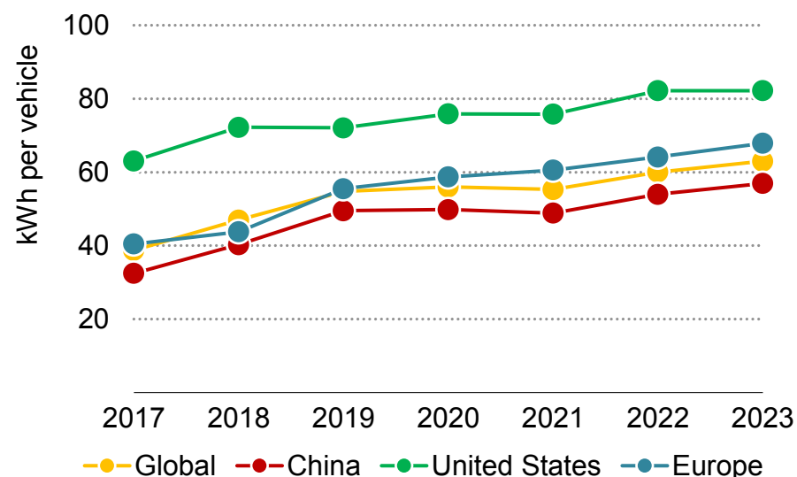
Average passenger BEV battery size, 2017-2023
