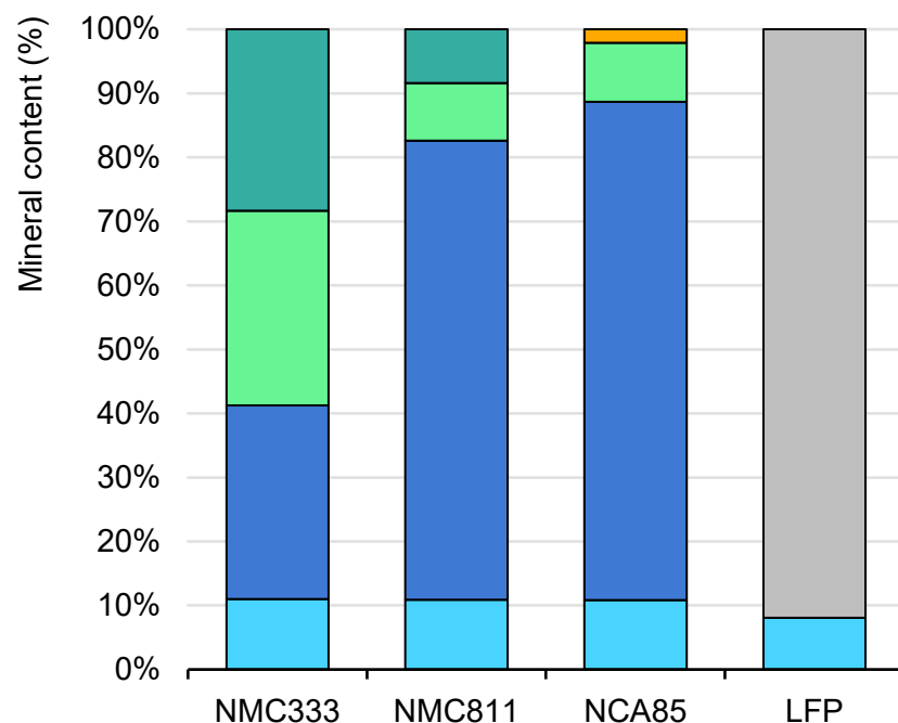
Mineral composition of different battery cathodes
