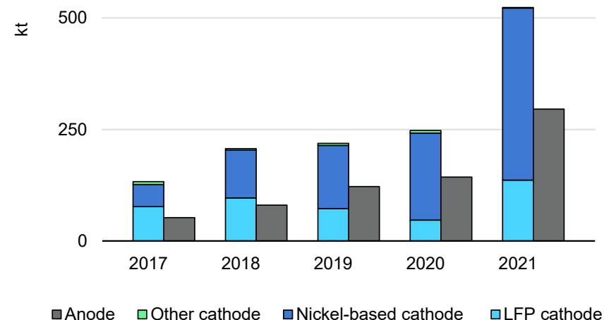
Battery cathode and anode material demand
