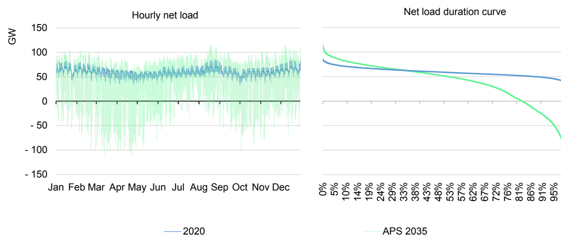
Hourly net load and load duration curve, 2020 and Announced Pledges Scenario 2035
