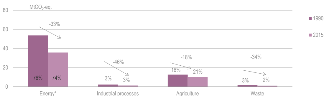
Figure 6.1 GHG emissions by sector, 1990 and 2015
