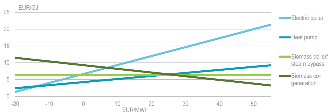
Figure 10.11 Marginal heat production cost by technology and by electricity price
