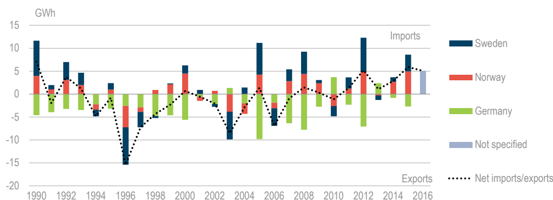
Figure 5.5 Electricity trade by country, 1990-2016
