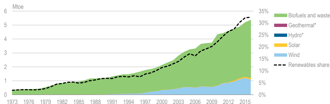
Figure 8.2 Renewable energy and waste in TPES, 1973-2016
